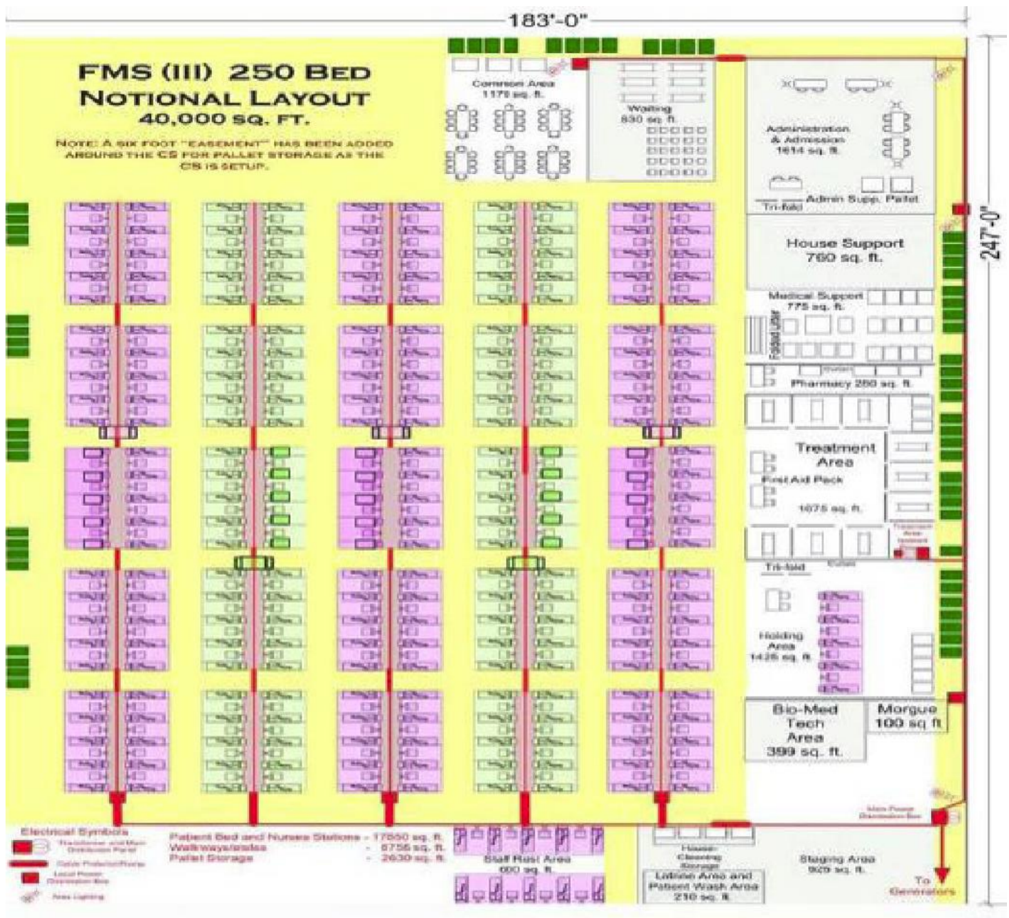
ACS Facility or Medical Needs Shelter Layout
